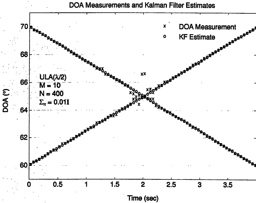
FIG. 12: Simulated SDMA Tracker Outputs — DOA Estimates and Kalman Filter Tracking of FM Transmitters Crossing Tracks in a Severe Rayleigh Fading Environment
